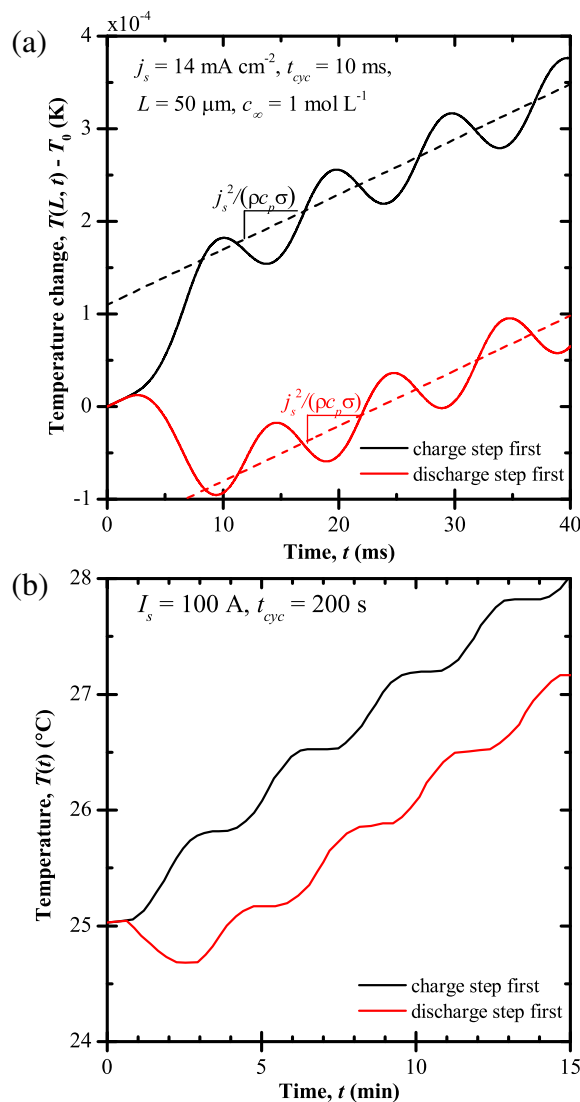
Fig. 9. (a) Numerically predicted temperature change T(L, t) - T_0 at the centerline and (b) measured surface temperature of a commercial EDLC (reproduced from Fig. 8 of Ref. [4]) as functions of time t for cases starting with either a charging step or a discharging step.
