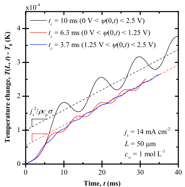
Fig. 11. Predicted temperature rise T(L,t) - T_0 as a function of time t at the centerline for cycling at the same current density j_s = 14 \text{ mA cm}^{-2} over different potential windows.
